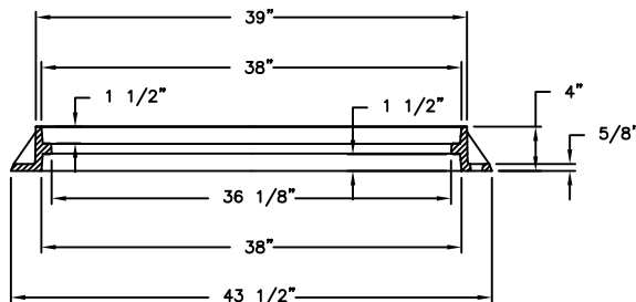
FRAME SECTION
