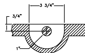
(4) TYPE 4 STAINLESS STEEL PICKBARS
