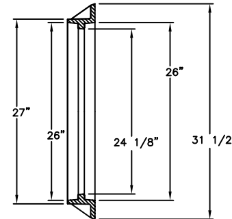
FRAME SECTION
